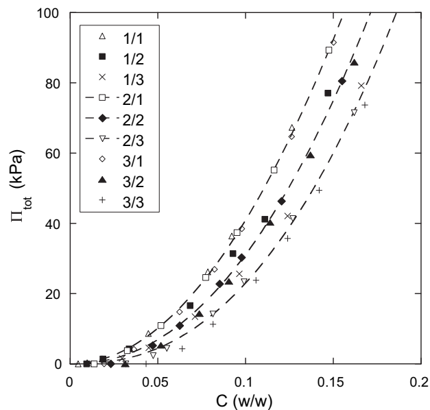
Fig. 3. Osmotic swelling pressure vs. total weight fraction of polymer for each of the nine hydrogels synthesized. The designation of each hydrogel, as defined in Table 1, is given in the legend. The dashed curves are drawn as a guide to the eyes and connect gels of the same crosslinker mole ratio. The experimental error of these measurements is comparable to the size of the symbols.
